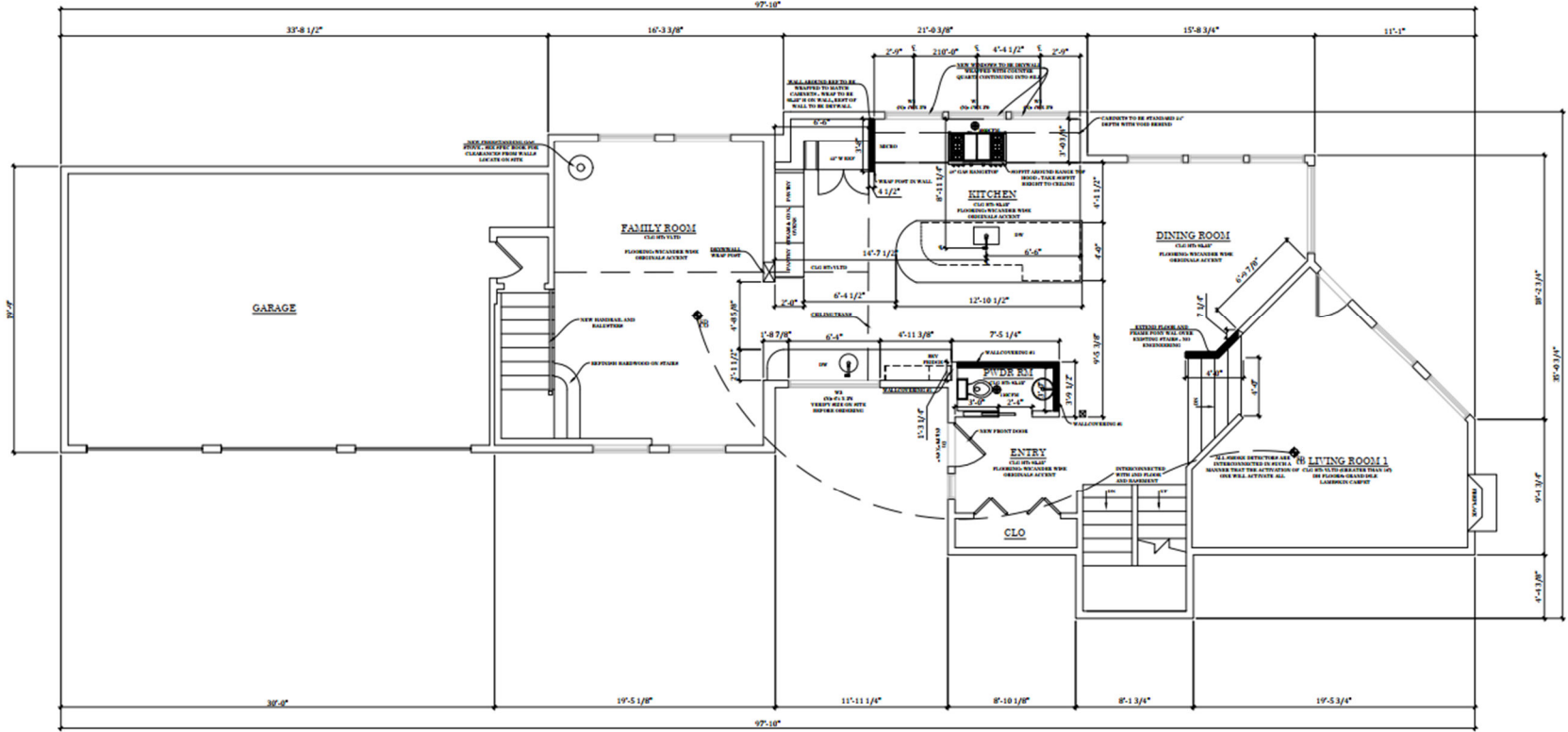
NEW MAIN FLOOR PLAN SCALE: 1/8" = 1'-0"
